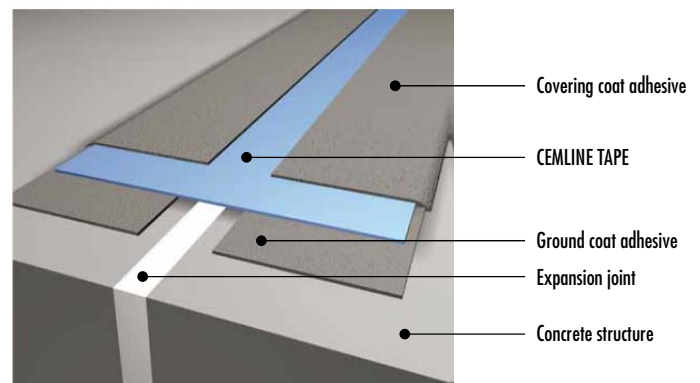
CEMLINE TAPE – Sealing of an expansion joint.
